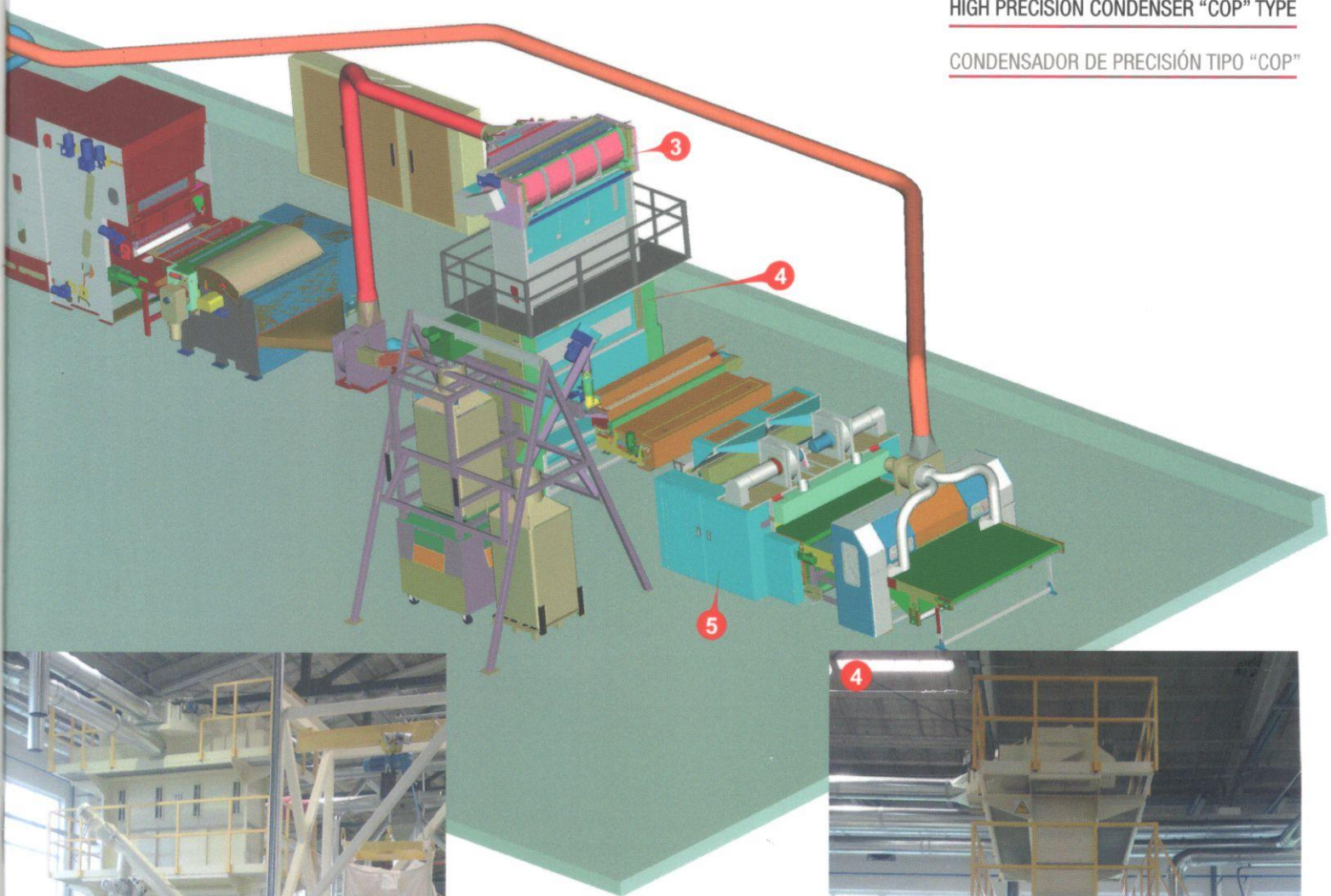
HIGH PRECISION CONDENSER "COP" TYPE
